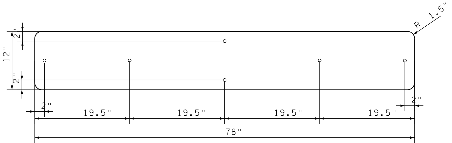
78" x 12" SIGN BLANK WITH 3/8" HOLES
