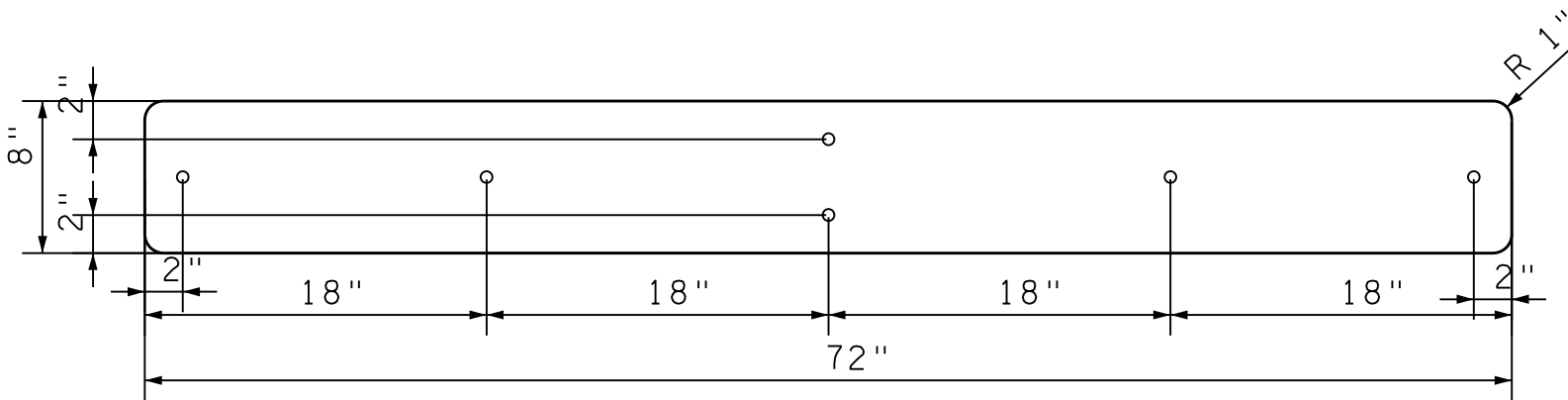
72" x 8" SIGN BLANK WITH 3/8" HOLES
