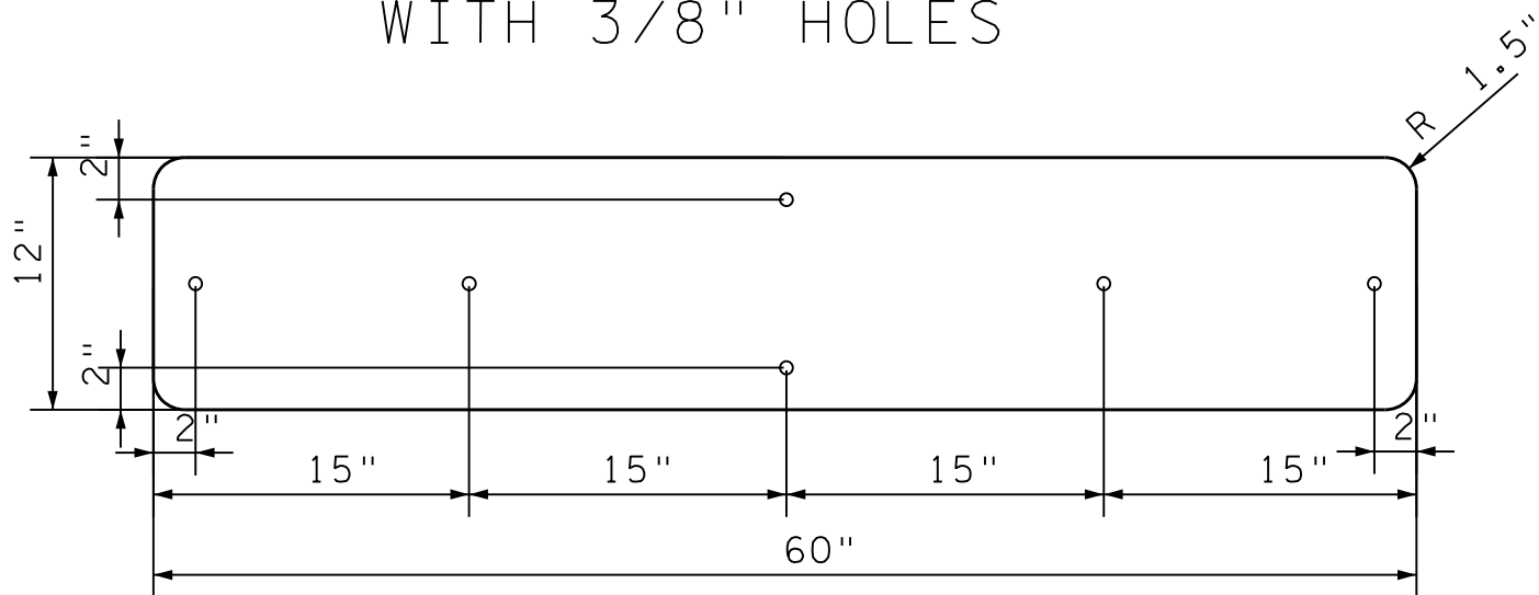
60" x 12" SIGN BLANK WITH 3/8" HOLES
