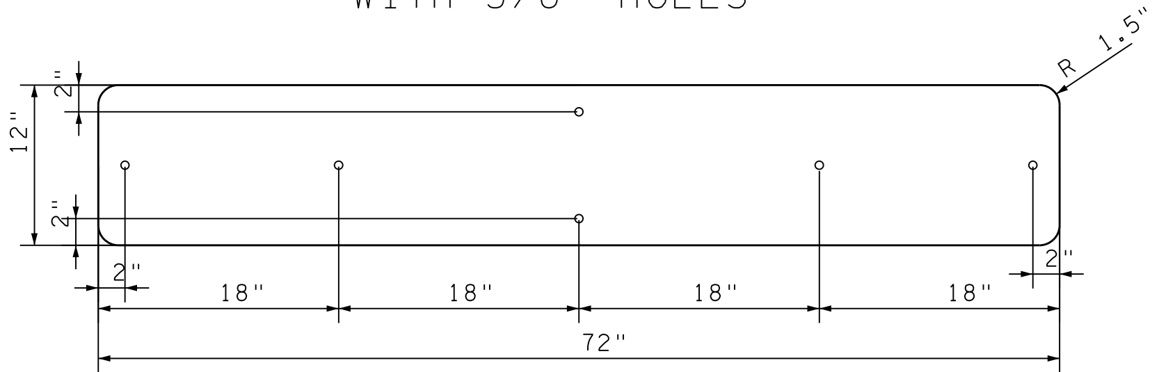
72" x 12" SIGN BLANK WITH 3/8" HOLES
