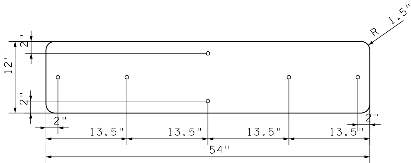
54" x 12" SIGN BLANK WITH 3/8" HOLES
