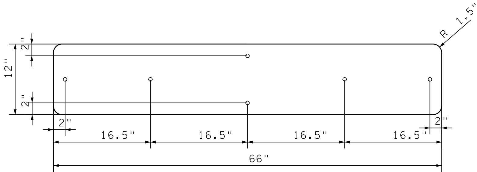
66" x 12" SIGN BLANK WITH 3/8" HOLES
