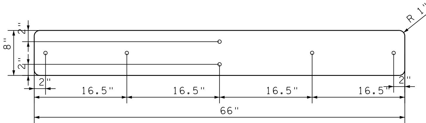
66" x 8" SIGN BLANK WITH 3/8" HOLES
