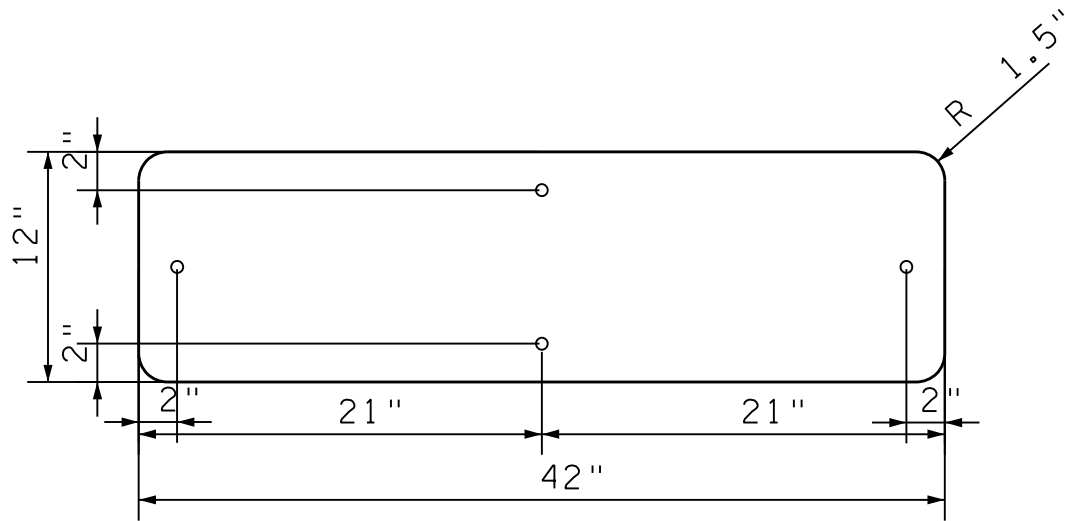
42" x 12" SIGN BLANK WITH 3/8" HOLES
